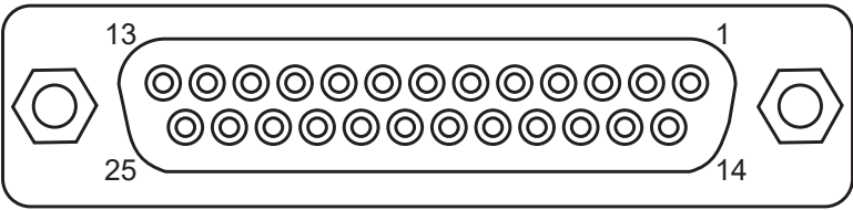
Connector pin-out
