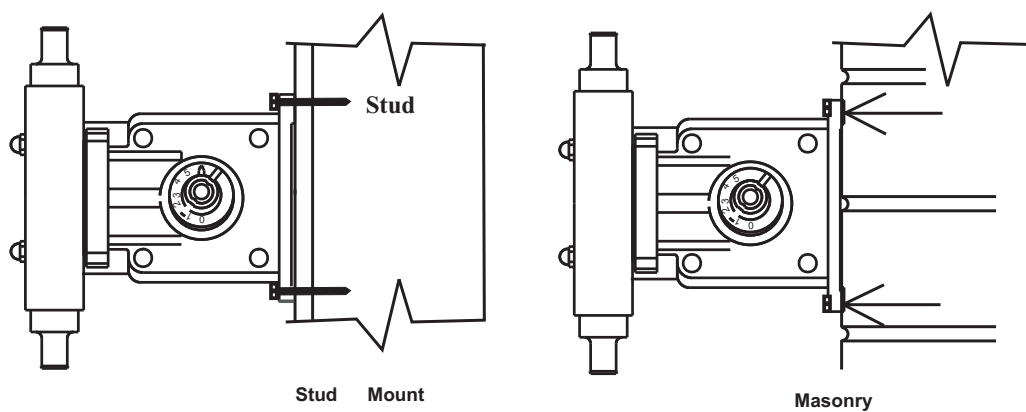
WALL MOUNTING
