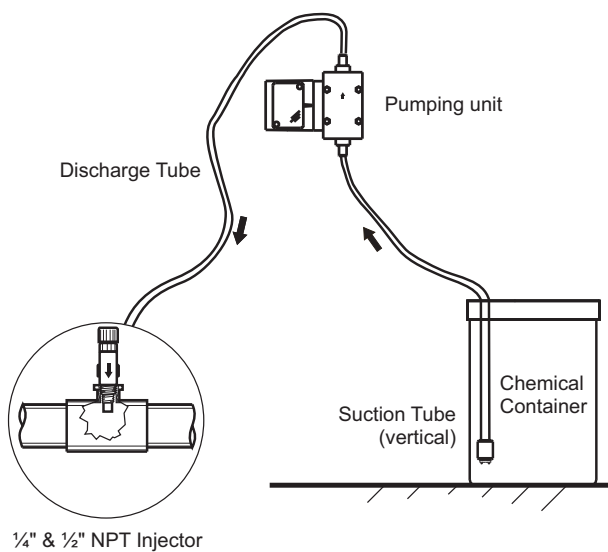
TYPICAL INSTALLATION
